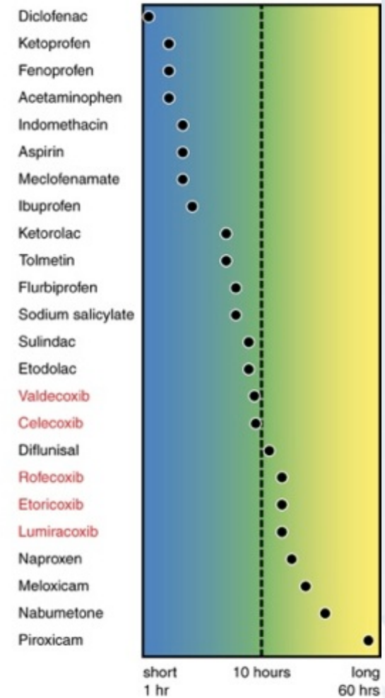
C Plasma t_{1/2} (log scale)
